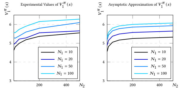
Figure 1: Comparison of experimental values and asymptotic approximation of V_1^\pi(s) .
