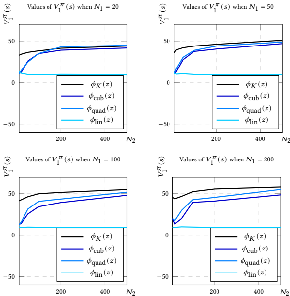
Figure 2: Comparison the values of V_1^\pi(s) between finite dimensional features and kernel features.
