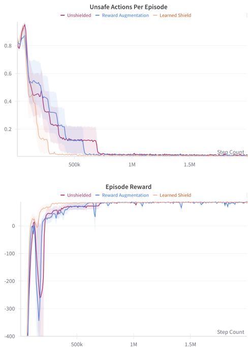
Figure 2: Average number of unsafe actions and reward per episode, and standard error over 10 trials for the gridworld-collision domain, “ISR” layout. Episode reward represents the original reward from the environment, prior to augmentation. Values are smoothed using a moving window average of 10K steps.
